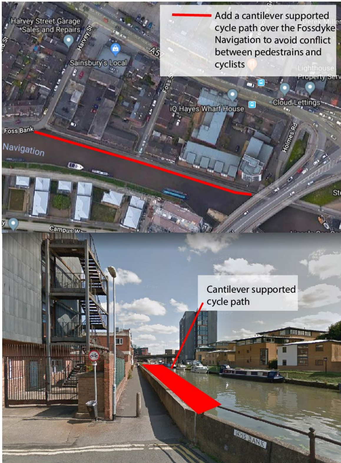
Figure 3: Cantilever cycle path over Fossdyke to keep cycle traffic off Carholme Road (Harvey Street to Holmes Road path)
